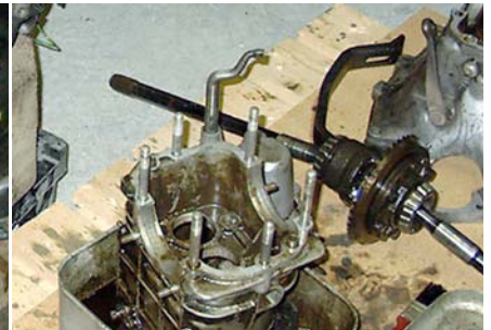
Differentialet adskilt, monteret nye pakdåser, ellers ok
